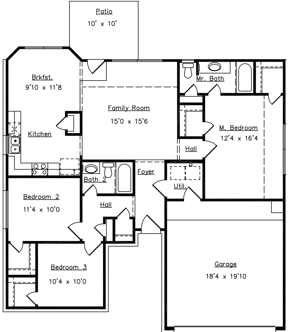
PLAN
